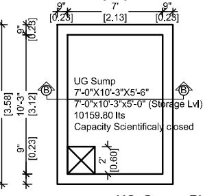
UG Sump Plan (Scale :Nts)
