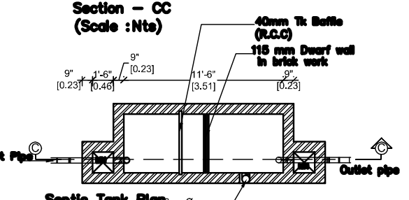
Septic Tank Plan (Scale :Nts)
