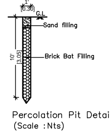
Percolation Pit Detail
