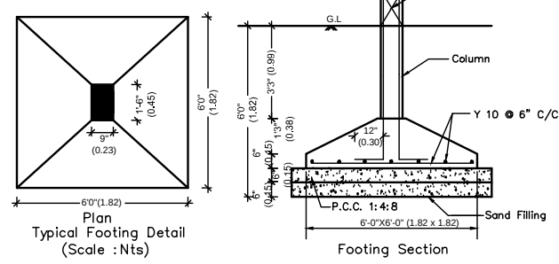
Typical Footing Detail
