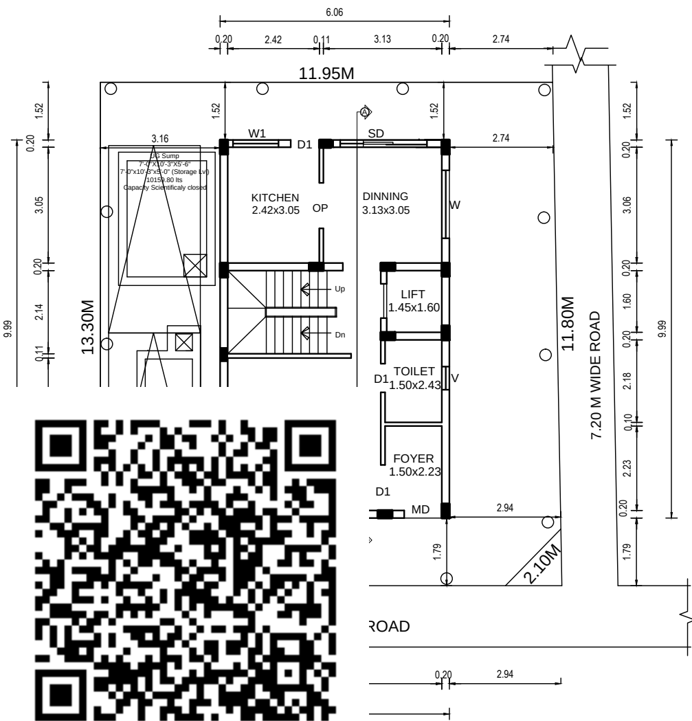
SITE CUM GROUND FLOOR PLAN
