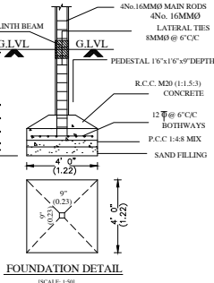
FOUNDATION DETAIL
