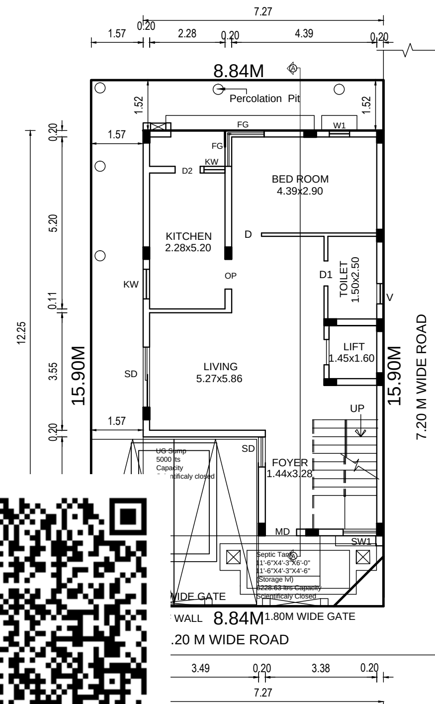
CUM GROUND FLOOR PLAN
