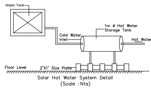
Solar Hot Water System Detail (Scale : Nts)
