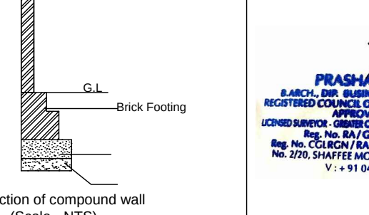
Section of compound wall (Scale - NTS)
