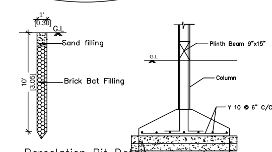
Percolation Pit Detail (Scale : Nts)
