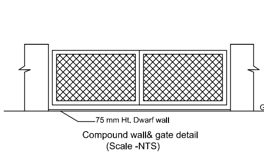
Compound wall & gate detail (Scale - NTS)
