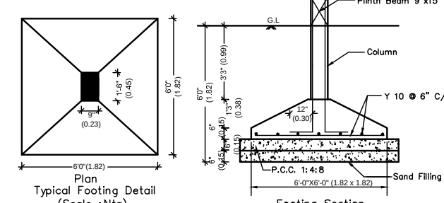
Typical Footing Detail
