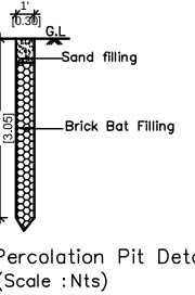
Percolation Pit Detail
