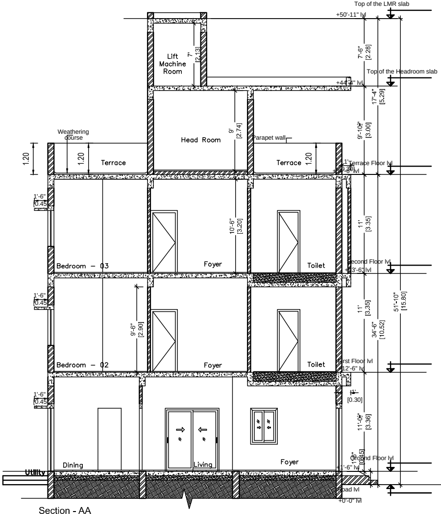
SECTION
