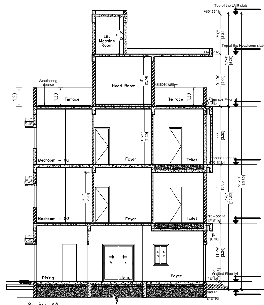
SECTION
