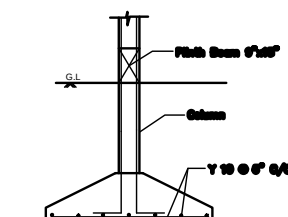
Foundation Detail (Scale : Nts)
