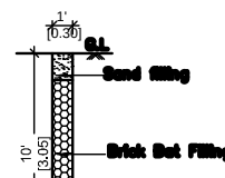
Percolation Pit Detail (Scale : Nts)
