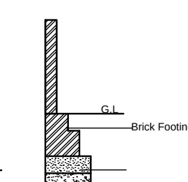
Section of compound wall (Scale : Nts)
