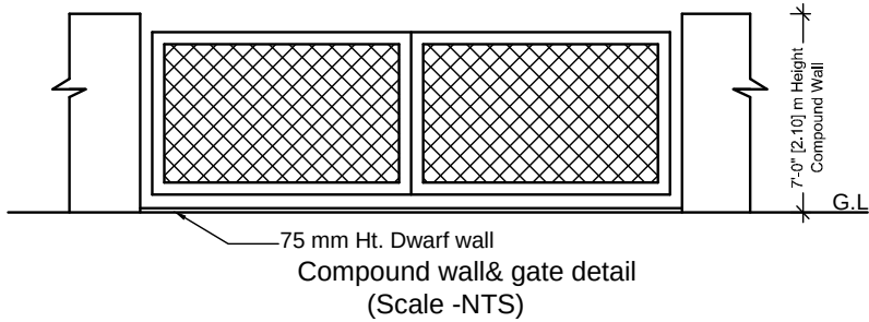
Section of compound wall (Scale - NTS)
