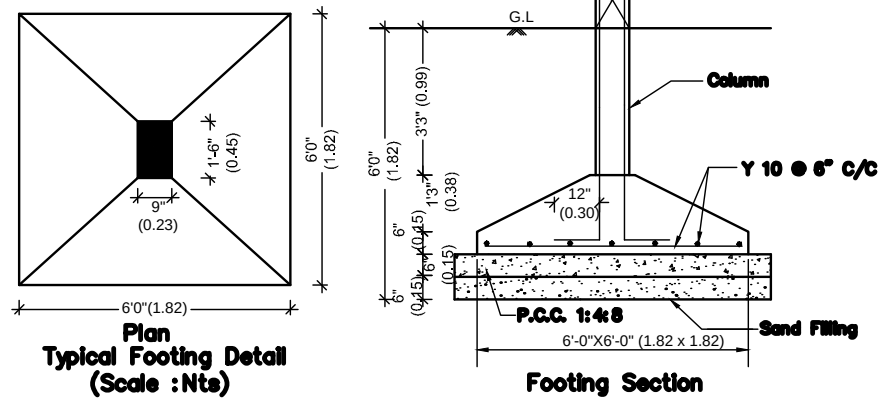
Footing Section
