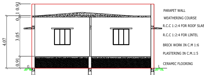
SECTION ON "SC"
