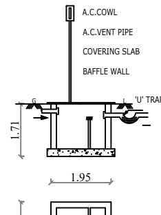
SEPTIC TANK
