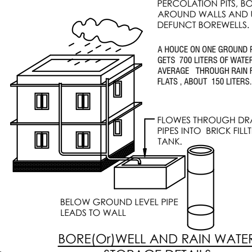
BORE(O)WELL AND RAIN WATER STORAGE DETAILS
