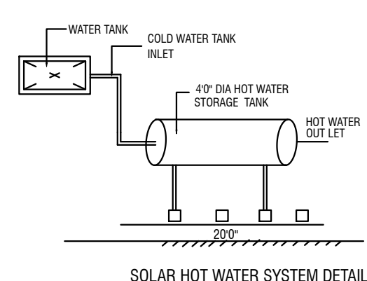
SOLAR HOT WATER SYSTEM DETAIL
