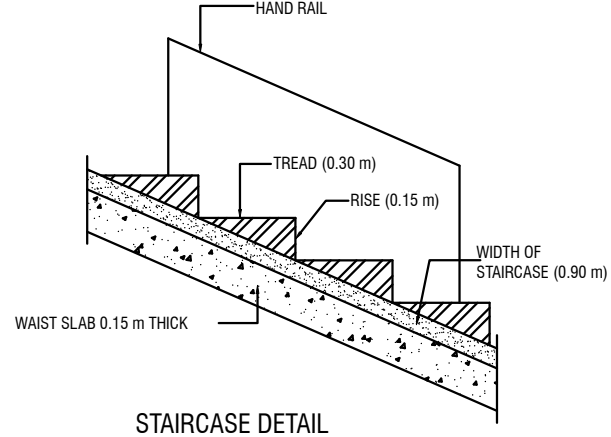
STAIRCASE DETAIL
