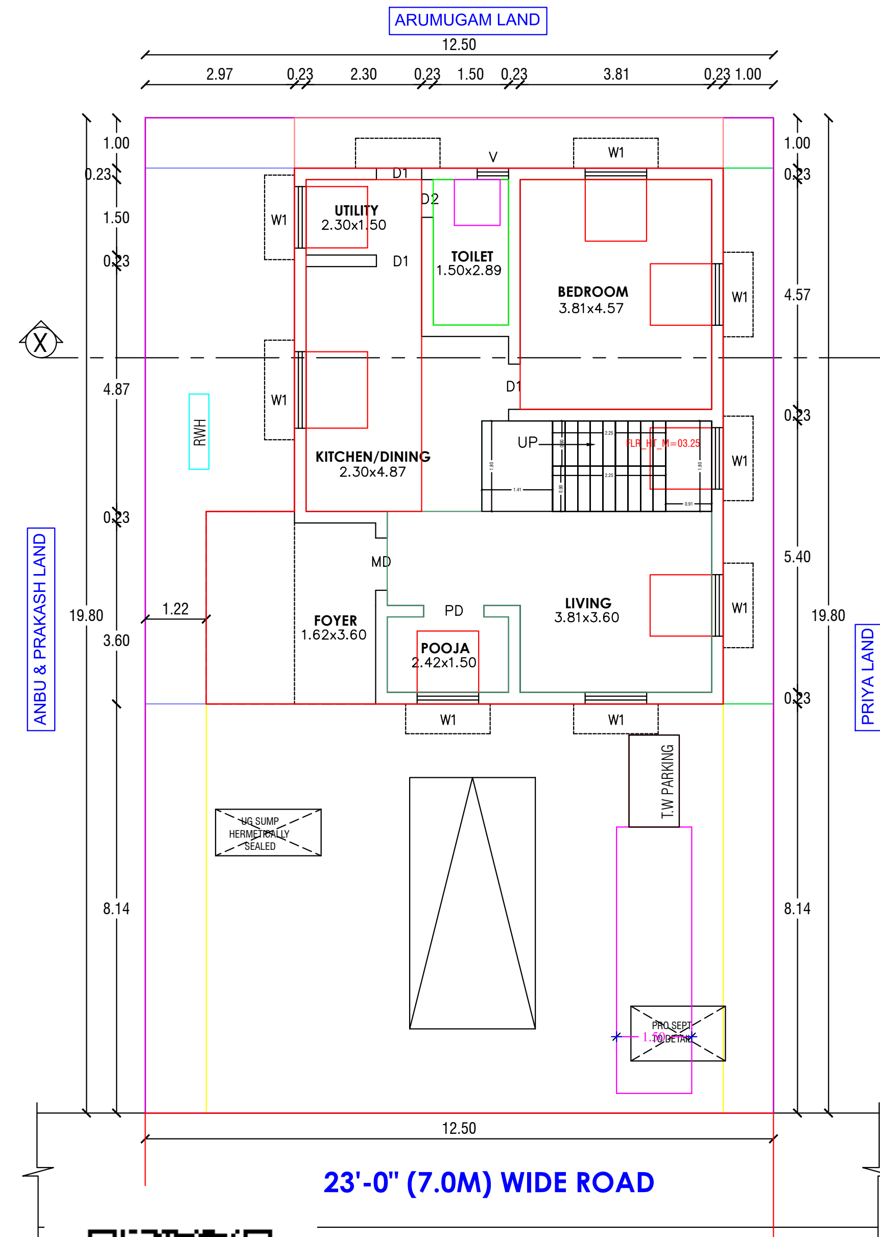
CUM GROUND FLOOR PLAN (PROPOSED)
