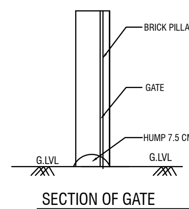
SECTION OF GATE
