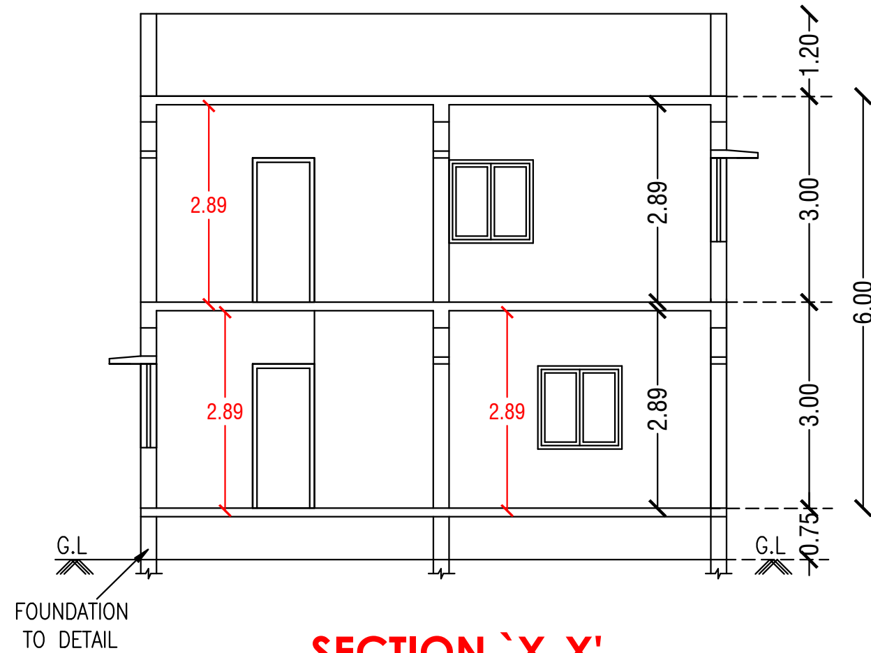
SECTION 'X-X'
