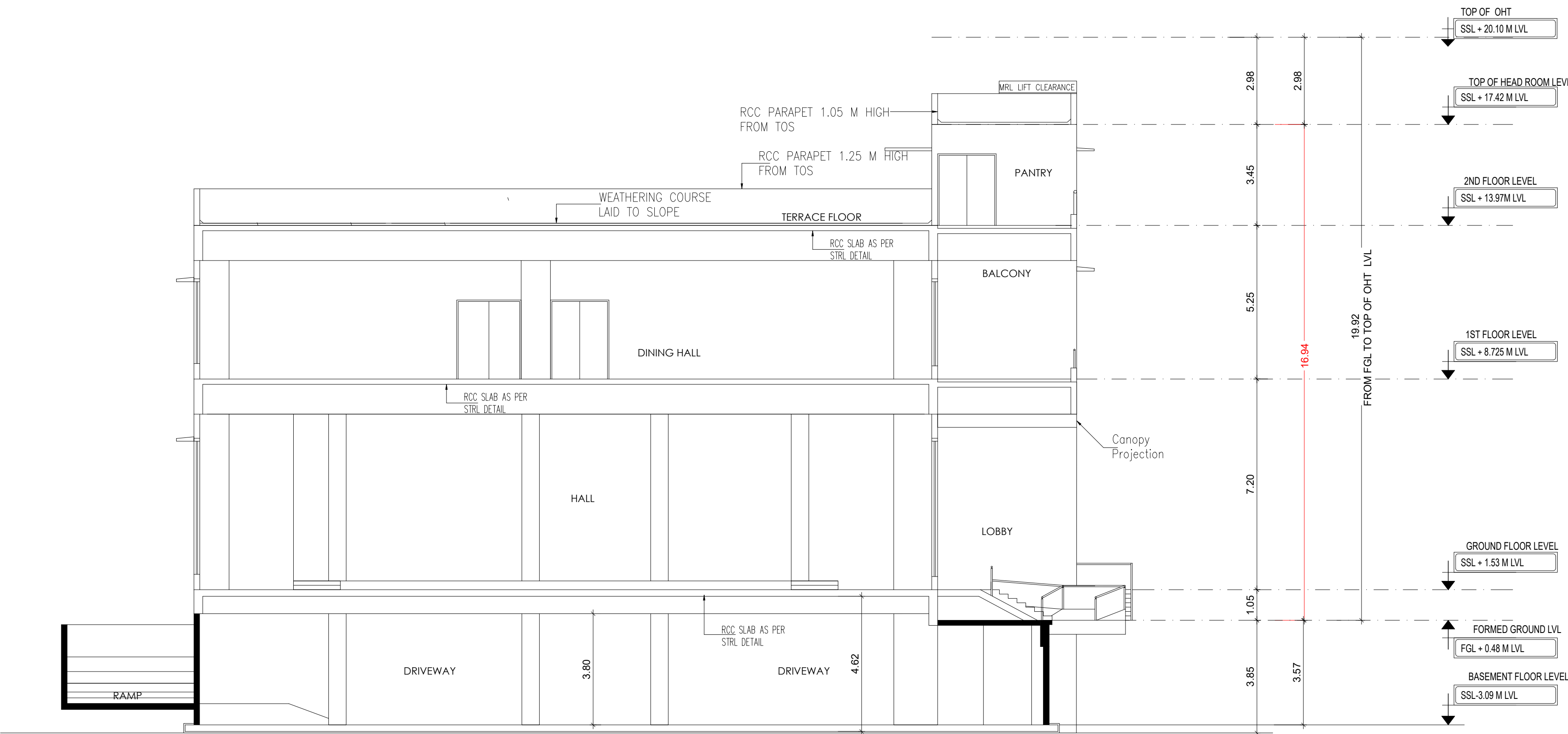
SECTION - BB
