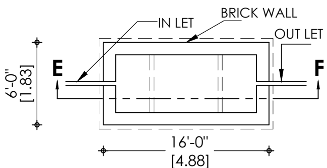
PLAN PLAN OF SEPTIC TANK
