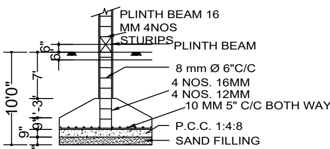
SECTION
