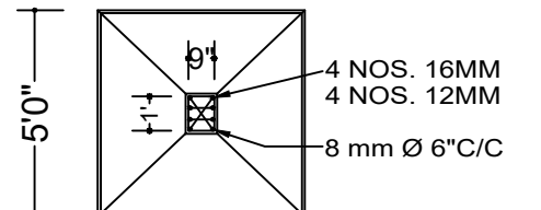
DETAIL OF COLUMN C1,C2
