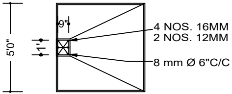
PLAN END WALL FOUNDATION
