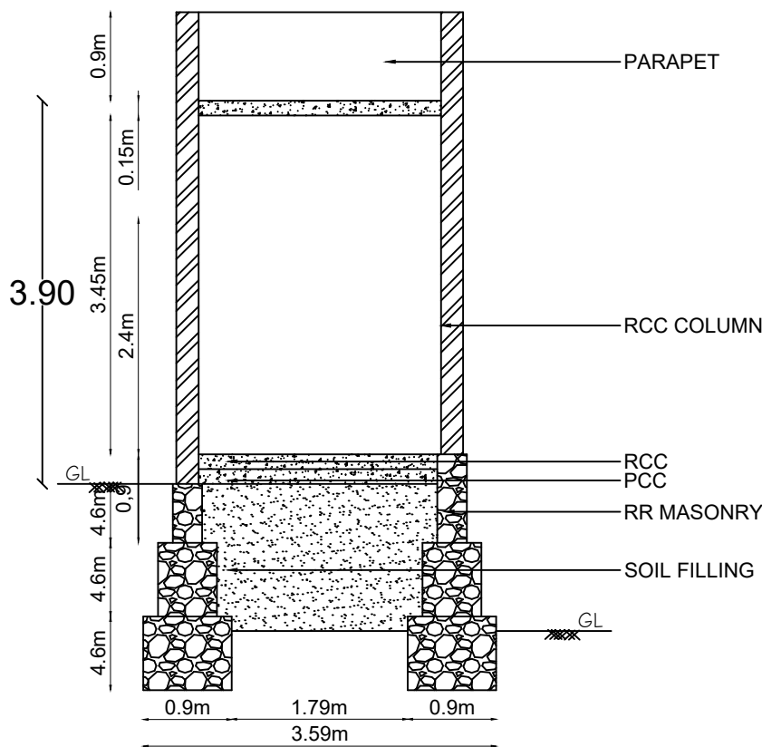
SECTIONAL VIEW X-X
