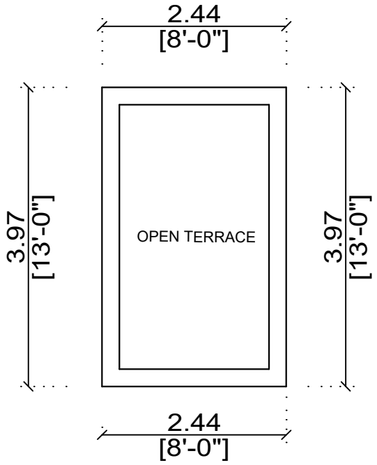
PRO.TERRACE FLOOR PLAN
