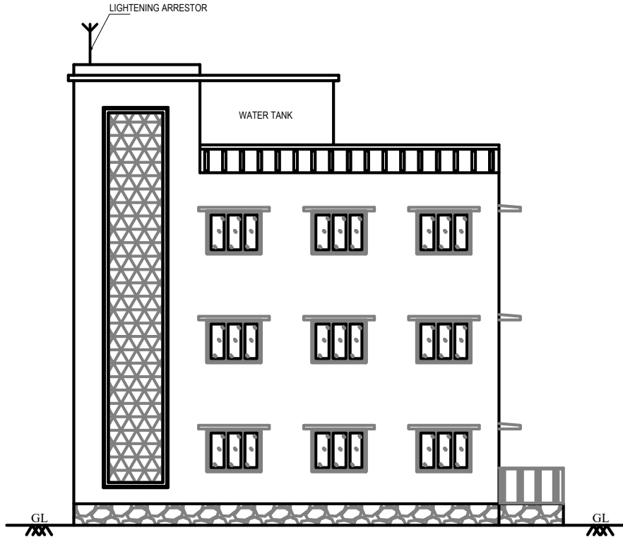
FRONT ELEVATION AT SOUTH SIDE
