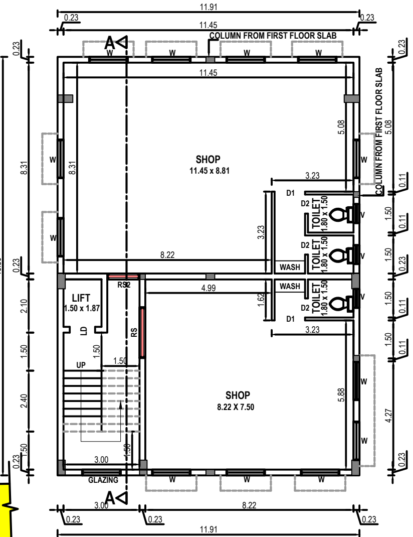
TYP. FIRST & SECOND FLOOR PLAN
