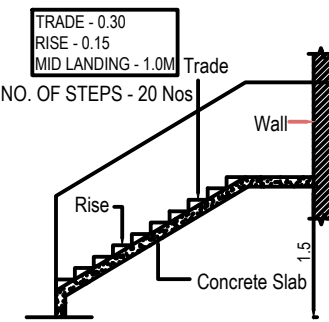
STAIR DETAILS
