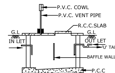
SEC. OF SEPTIC TANK
