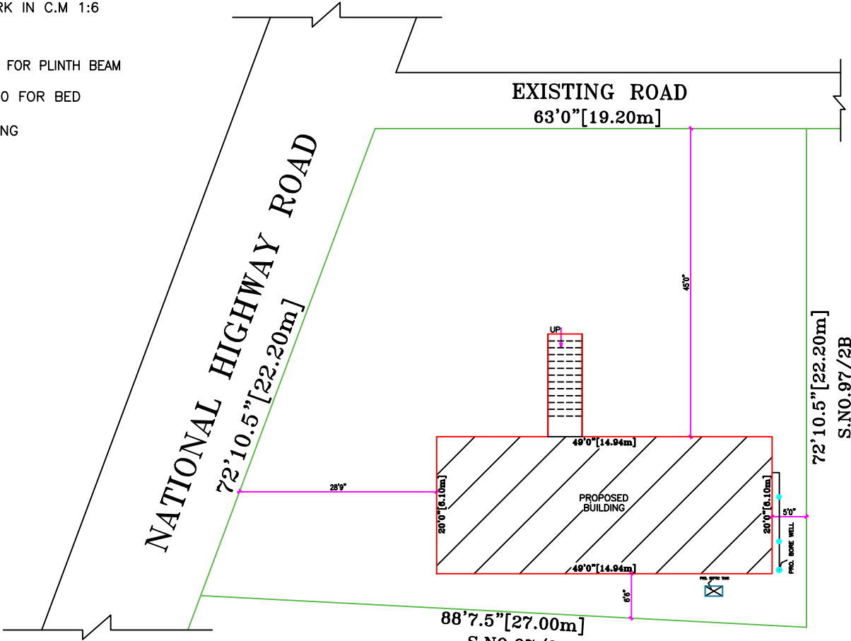
SITE PLAN
