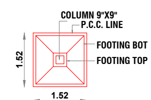
PLAN OF FOOTING
