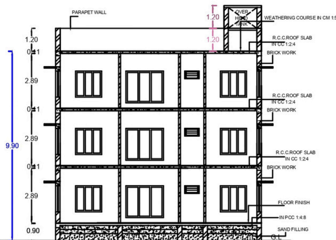
SECTION "AA"
