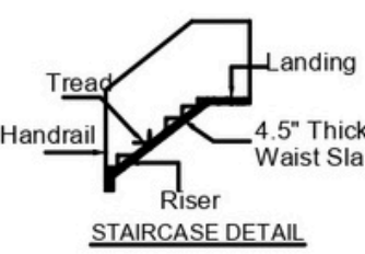
STAIRCASE DETAIL
