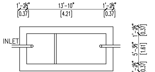
DETAILS OF SEPTIC TANK
