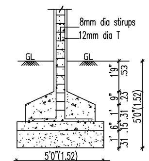
SCALE 1"=4'0" (1:50) COLUMN FOUNDATION DETAIL
