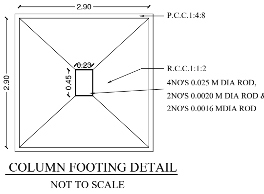
FOUNDATION DETAIL
