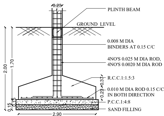
FOUNDATION DETAIL
