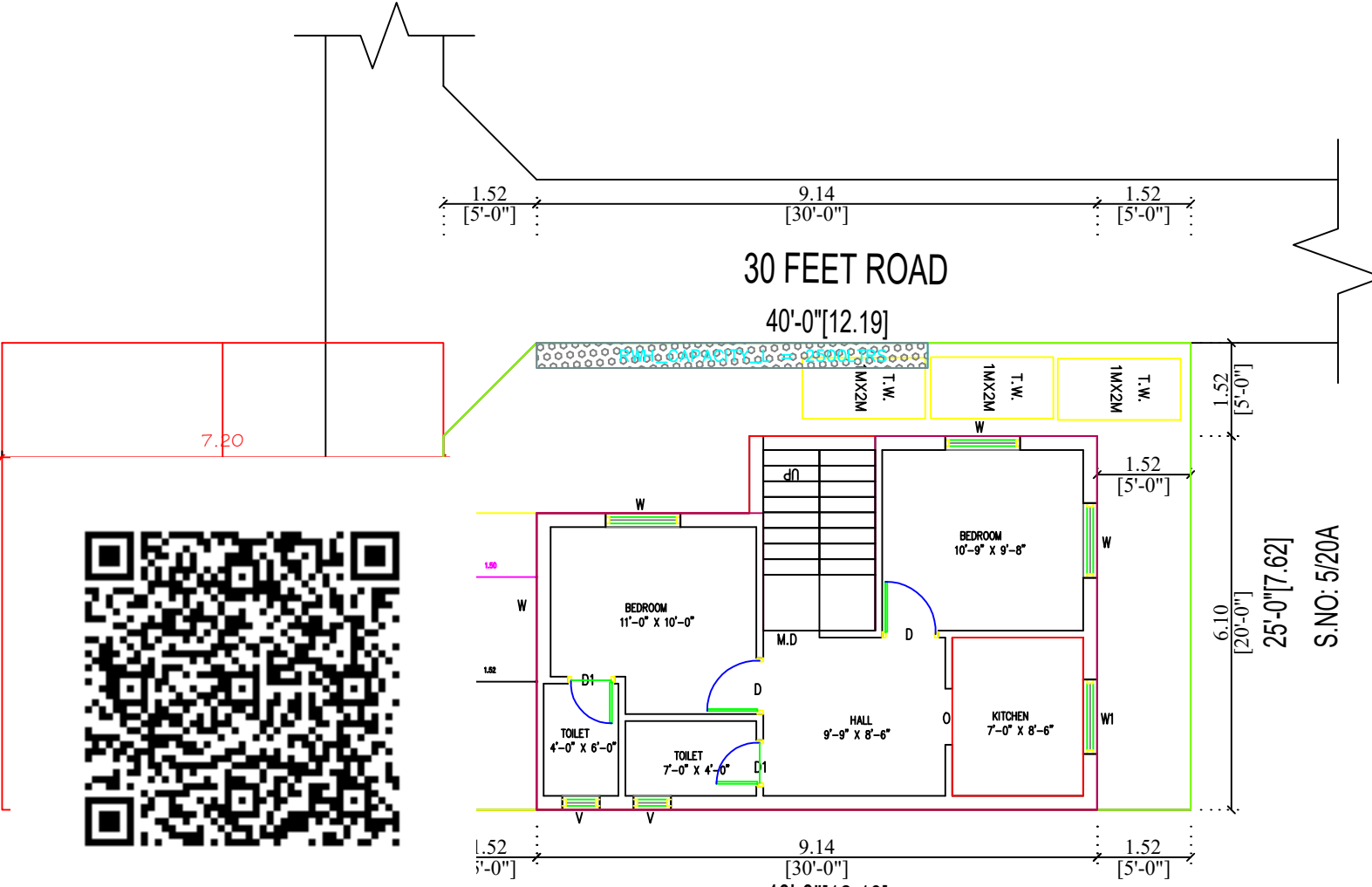
PLOT NO: 7 SITE CUM GROUND FLOOR PLAN
