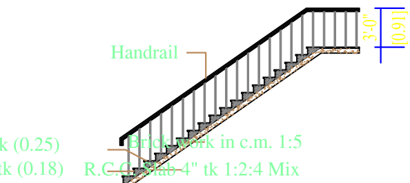
Staircase Details
