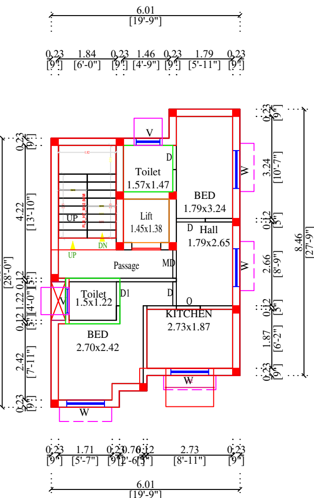
FIRST FLOOR PLAN TYPICAL_FLOOR_PLAN=1,2,3
