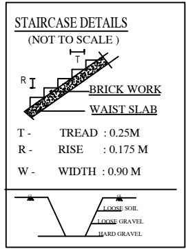
STAIRCASE DETAILS
