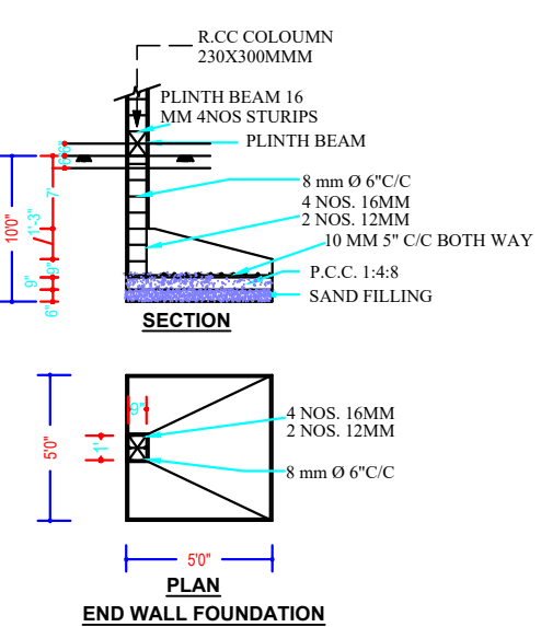
END WALL FOUNDATION
