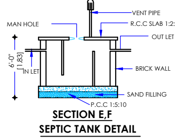
SECTION E.F
