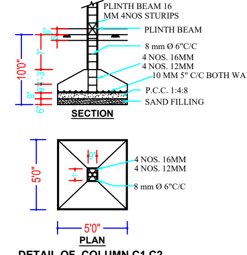
DETAIL OF COLUMN C1,C2
