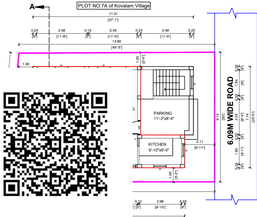
SITE CUM GROUND FLOOR PLAN (PROPOSED)
