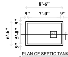
PLAN OF SEPTIC TANK
