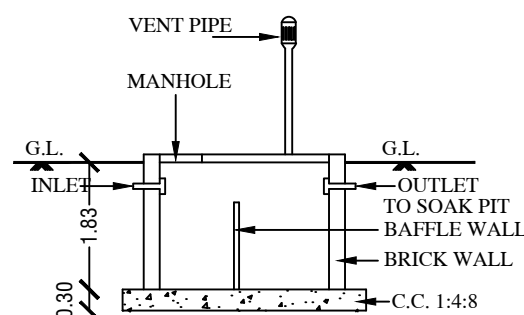
SECTION OF SEPT. TANK
