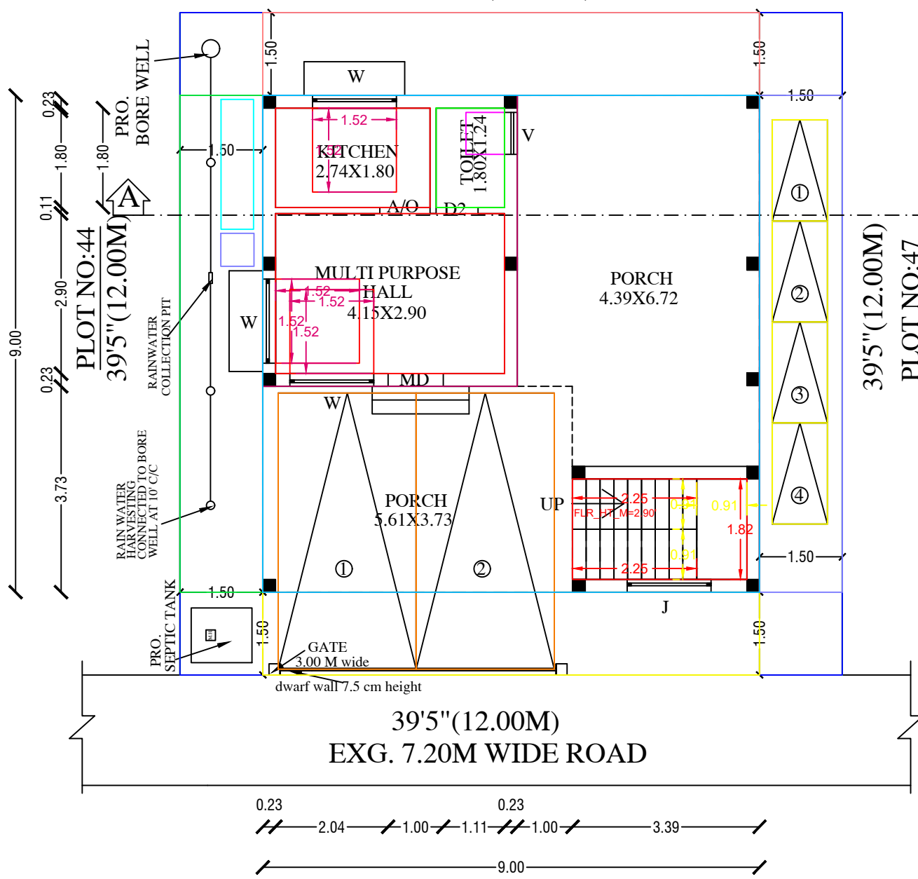
SITE PLAN CUM FLOOR PLAN
