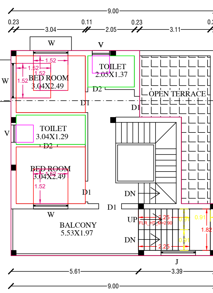
SECOND FLOOR PLAN (PART)
