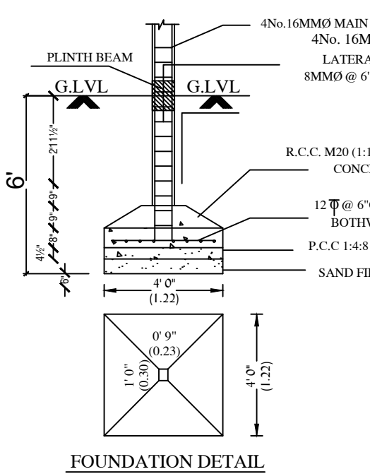
FOUNDATION DETAIL (SCALE:1:50)
