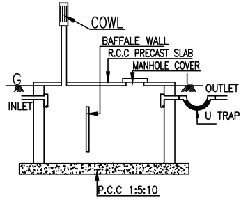
DETAILS OF SEPTIC TANK
