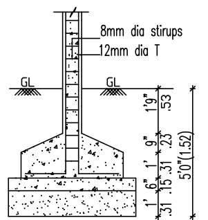
COLUMN FOUNDATION DETAIL SCALE 1"=4'0"(1:50)
