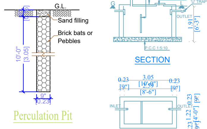
PLAN DETAILS OF SEPTIC TANK
