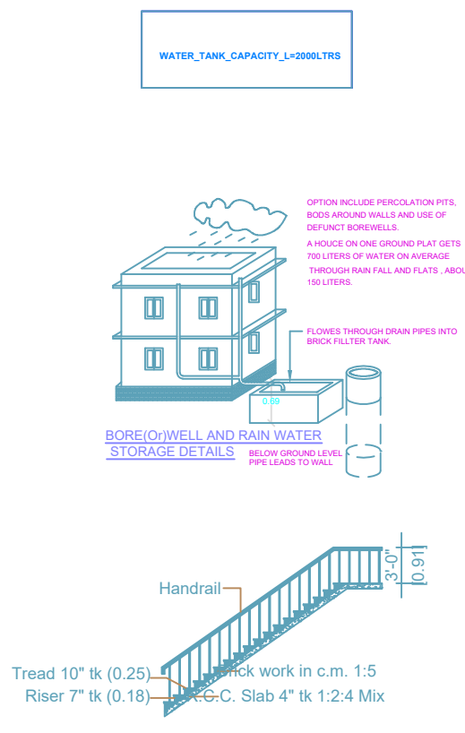
Staircase Details
