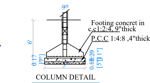
COLUMN DETAIL
