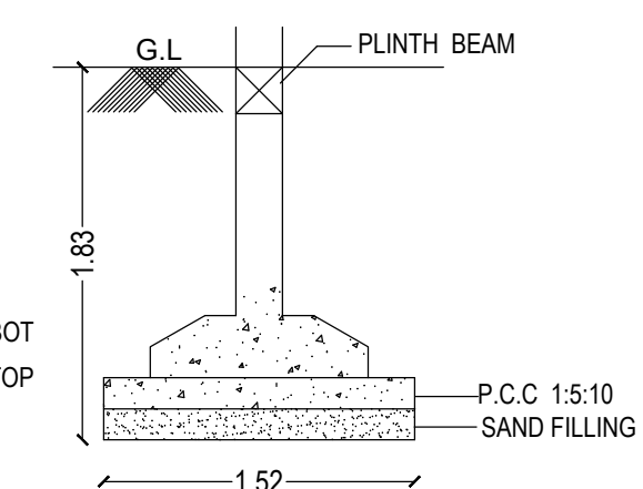
FOUNDATION DETAIL
