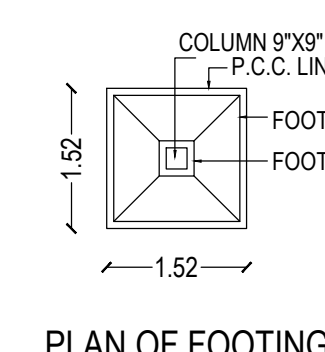
PLAN OF FOOTING
