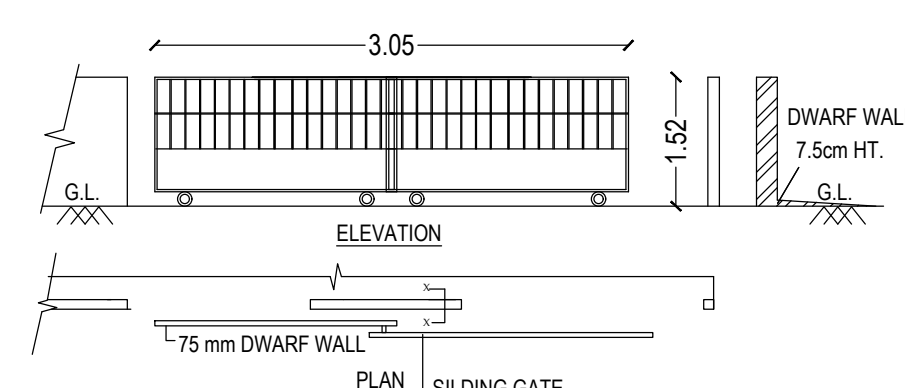
COMPOUND WALL & GATE DETAIL NOT TO SCALE
