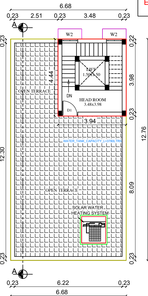
TEERACE FLOOR PLAN (PROPOSED)
