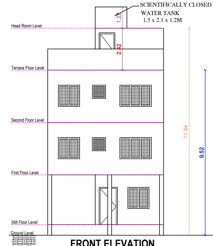
FRONT ELEVATION (PROPOSED)
