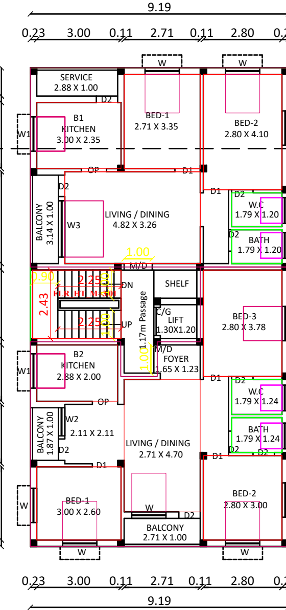
PRO.SECOND FLOOR PLAN
