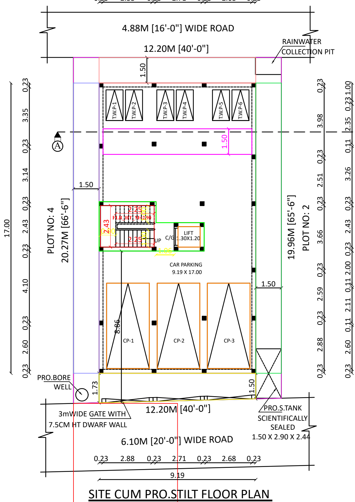
SITE CUM PRO.STILT FLOOR PLAN
