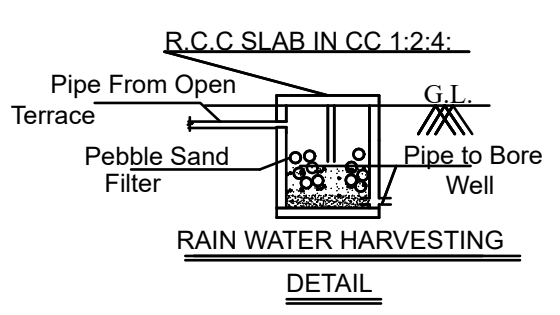
RAIN WATER HARVESTING DETAIL
