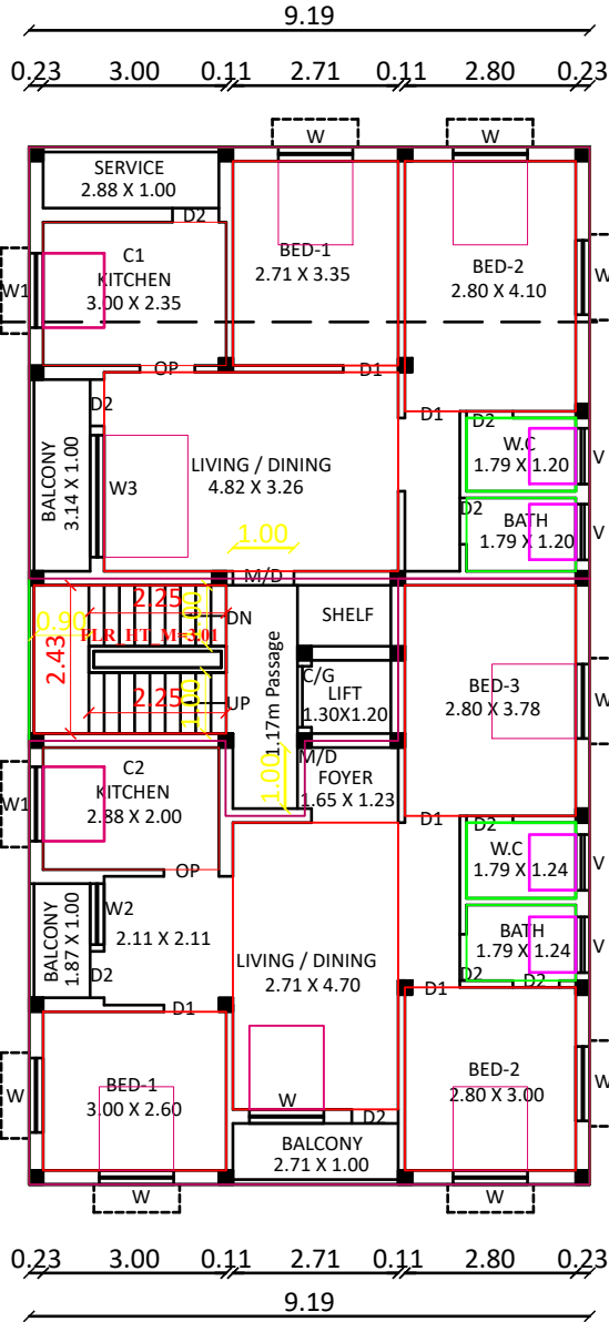
PRO.THIRD FLOOR PLAN
