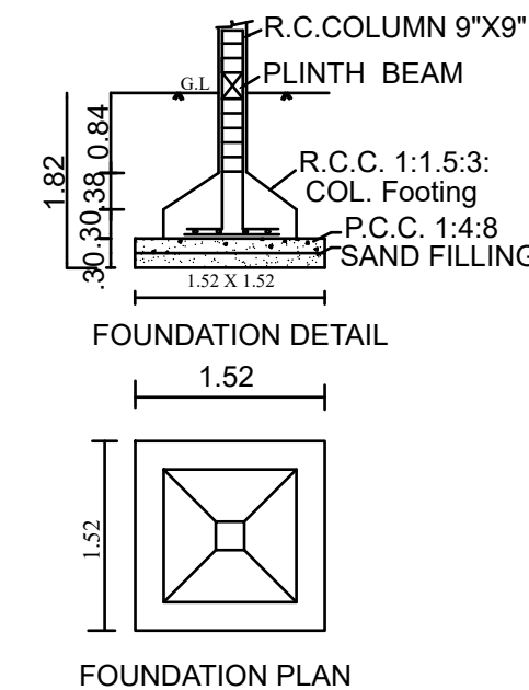
FOUNDATION DETAIL
