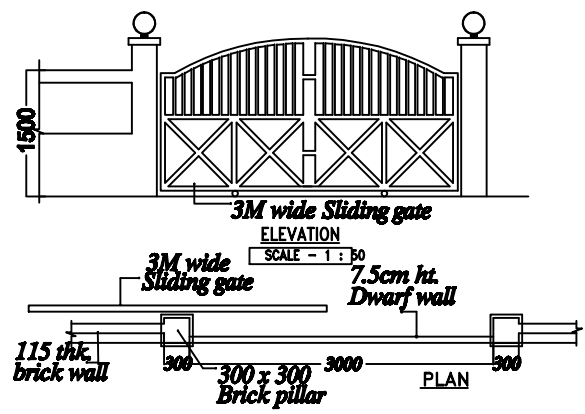
COMPOUND WALL DETAIL
