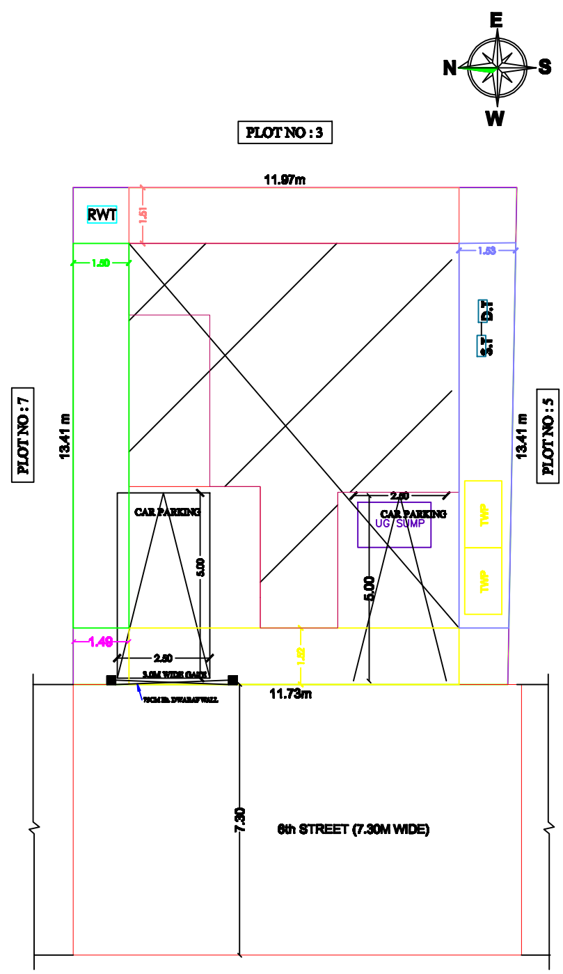
SITE PLAN
