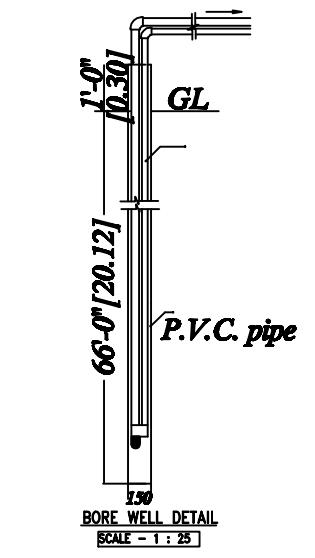
SIZE:- 9" X 1'-3"
