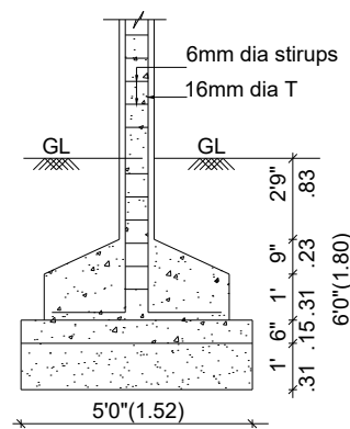
COLUMN FOUNDATION DETAIL SCALE (1:50)
