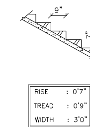
STAIR DETAILS
