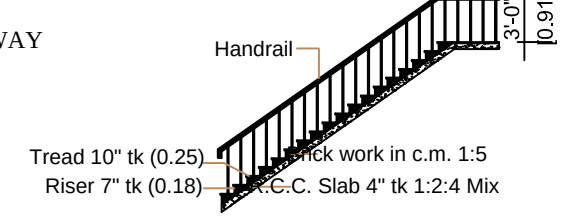
Staircase Details
