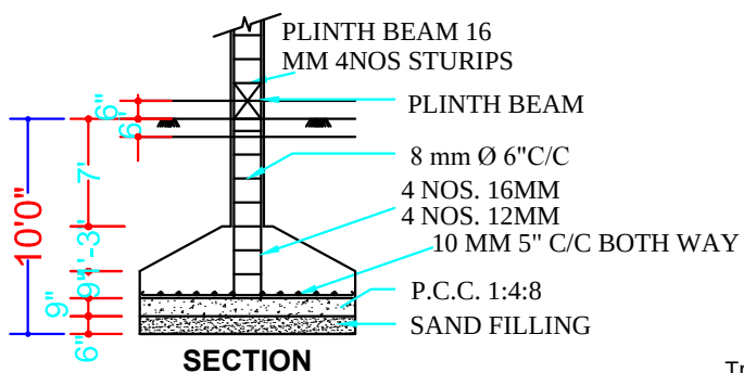
SECTION
