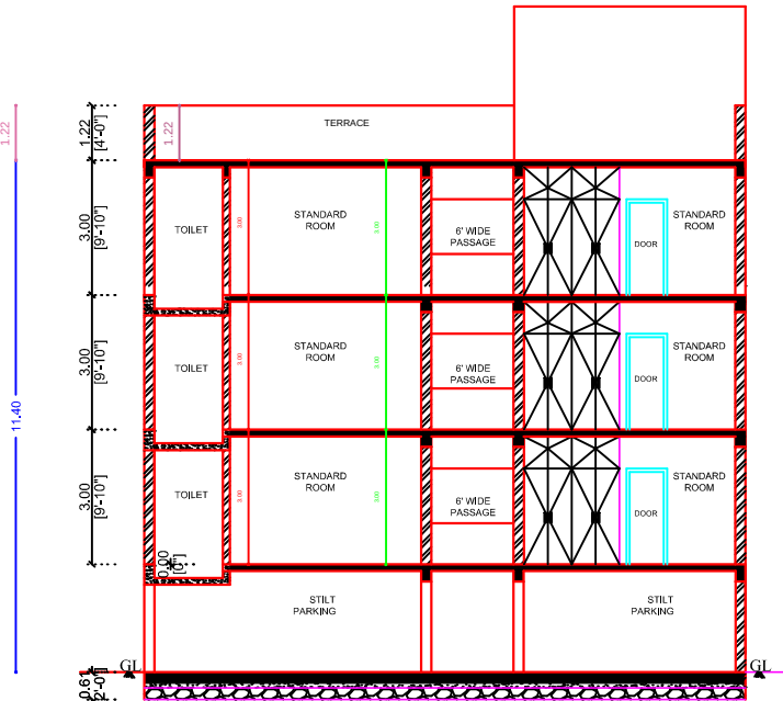
SECTION A
