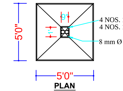
PLAN DETAIL OF COLUMN C1,C2
