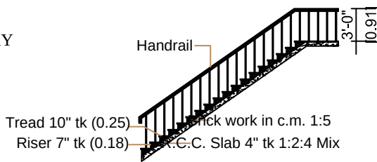
Staircase Details
