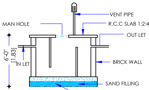
SECTION E,F SEPTIC TANK DETAIL
