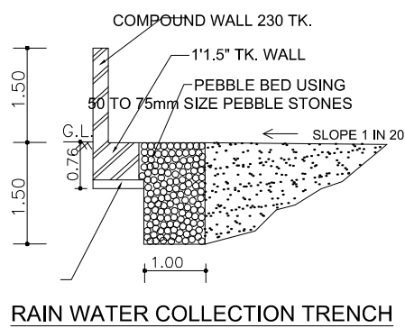
RAIN WATER COLLECTION TRENCH
