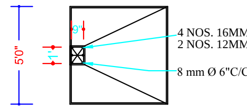
PLAN END WALL FOUNDATION
