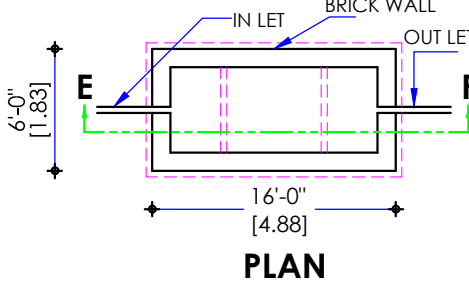
PLAN PLAN OF SEPTIC TANK
