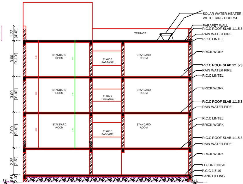
SECTION A
