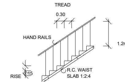
STAIRCASE DETAILS
