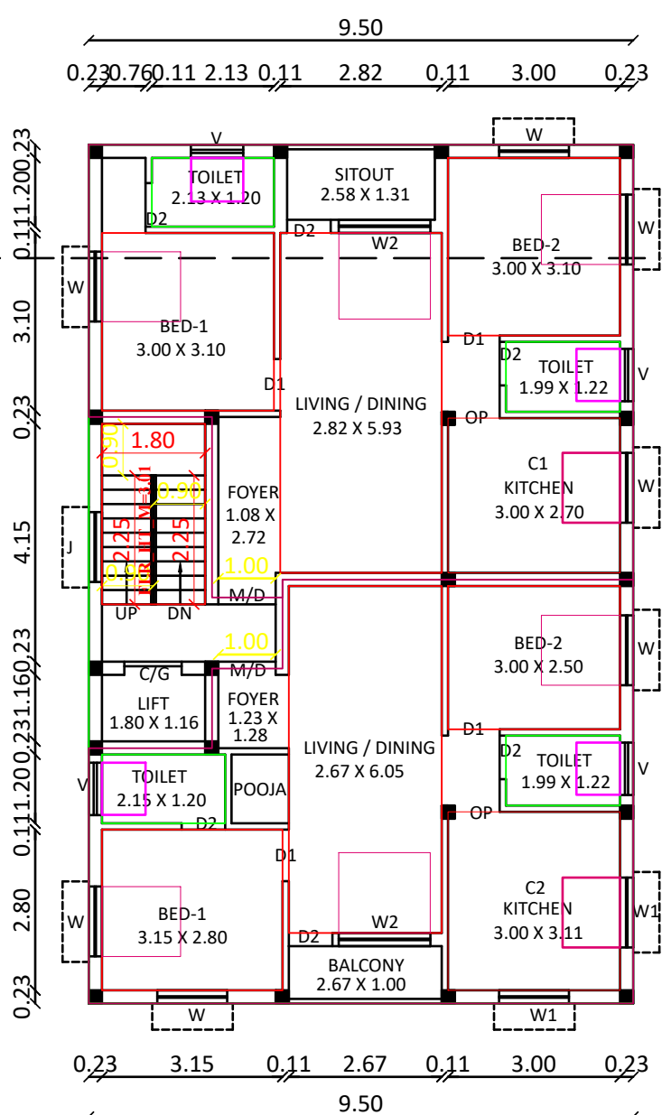
PRO.THIRD FLOOR PLAN
