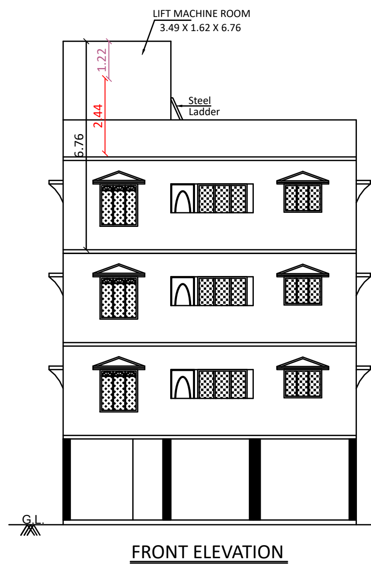
FRONT ELEVATION
