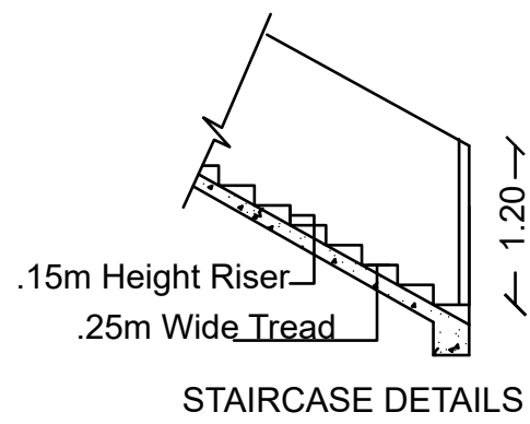
STAIRCASE DETAILS
