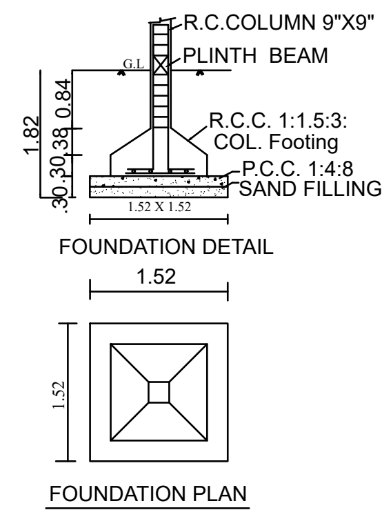
FOUNDATION PLAN
