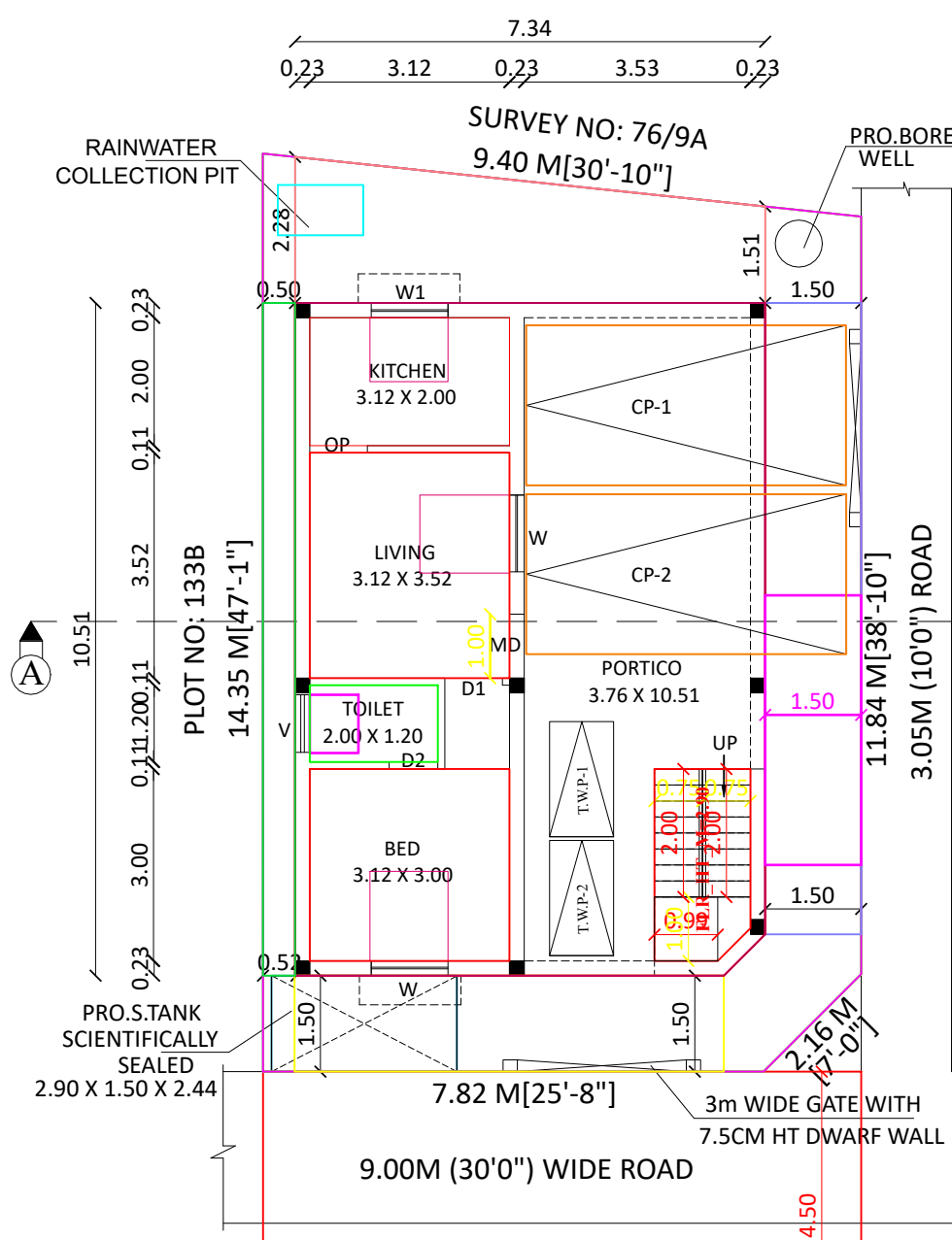
ROUND FLOOR PLAN
