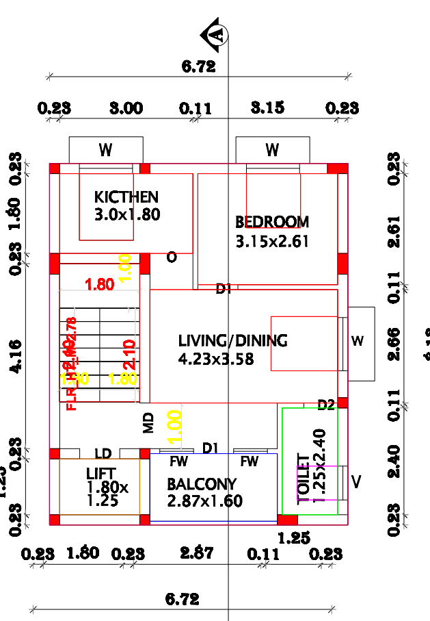
TYPICAL FLOOR PLAN OF I, II & III TYPICAL_FLOOR_PLAN=1,2,3
