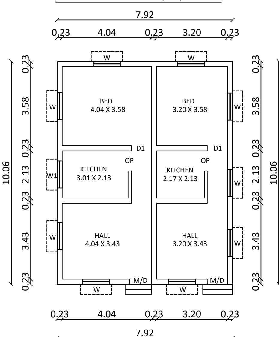
EXG.GROUND FLOOR PLAN
