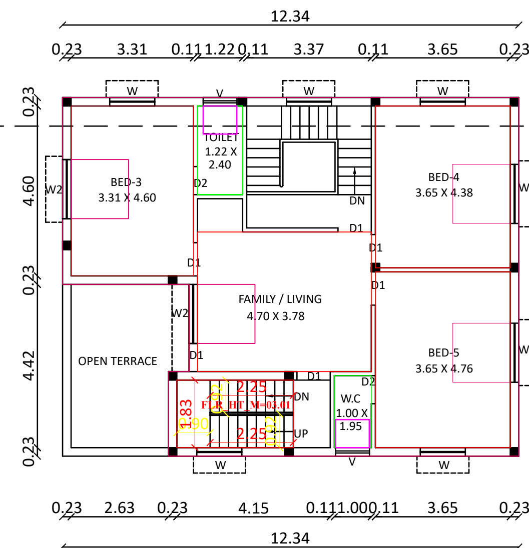
PRO.FIRST FLOOR(PT) PLAN
