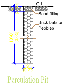
Percolation Pit
