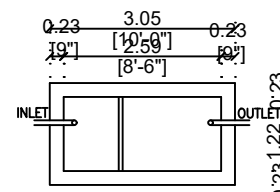
PLAN DETAILS OF SEPTIC TANK
