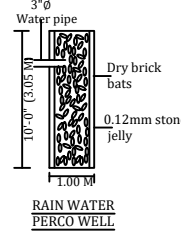
SECTION OF SOAKAGE PIT
