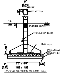
TYPICAL SECTION OF FOOTING
