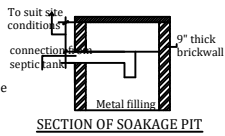
SECTION OF SOAKAGE PIT
