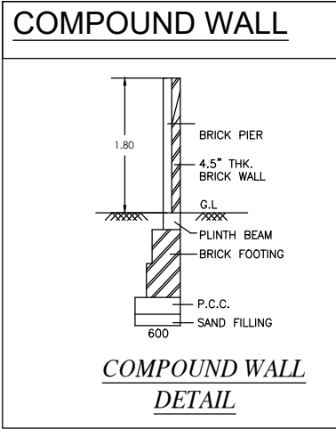
COMPOUND WALL
