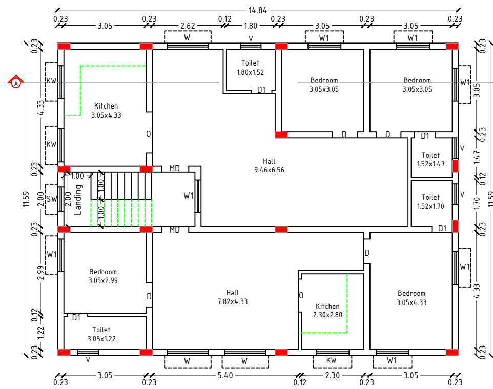
TYPICAL FLOOR PLAN FIRST, SECOND & THIRD
