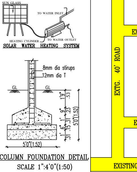
COLUMN FOUNDATION DETAIL
