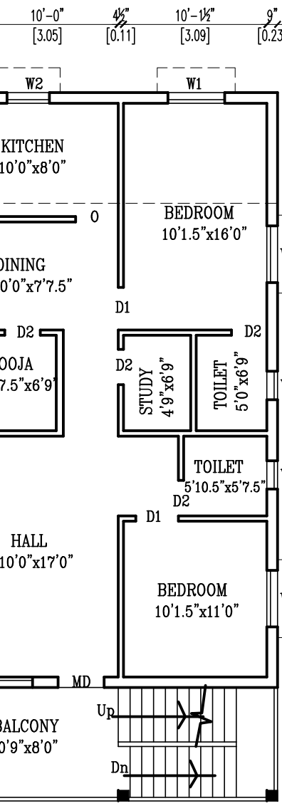
EXTG. FIRST FLOOR PLAN
