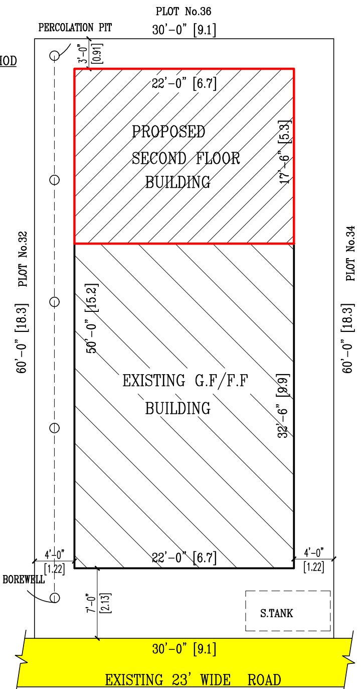
SITE PLAN
