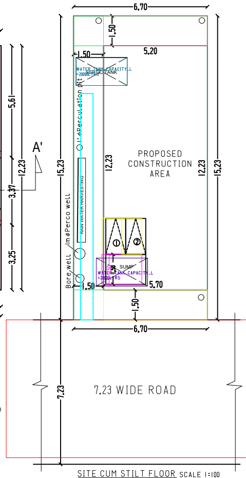
SITE CUM STILT FLOOR SCALE 1:100
