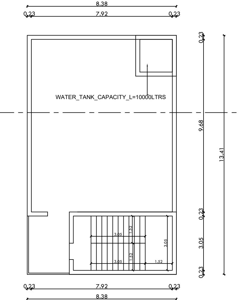
Pro. Terrace Floor Plan
