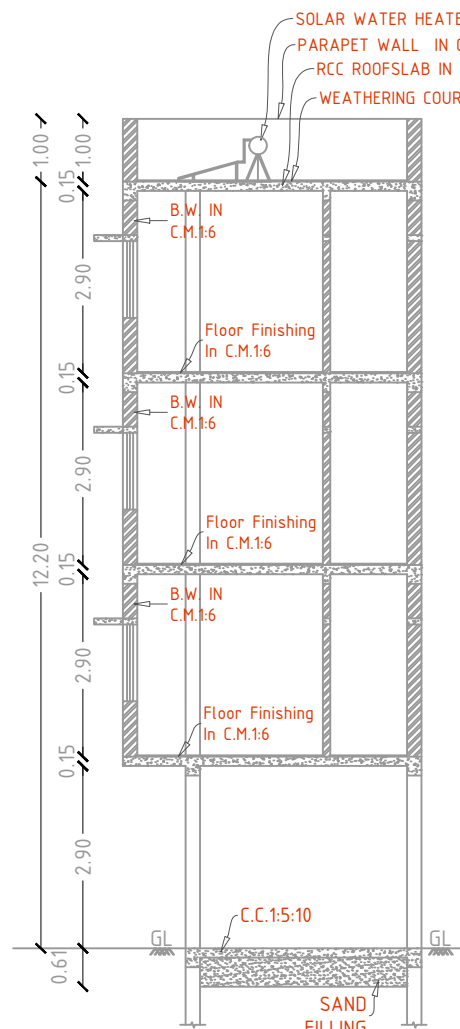
SECTION-A-A
