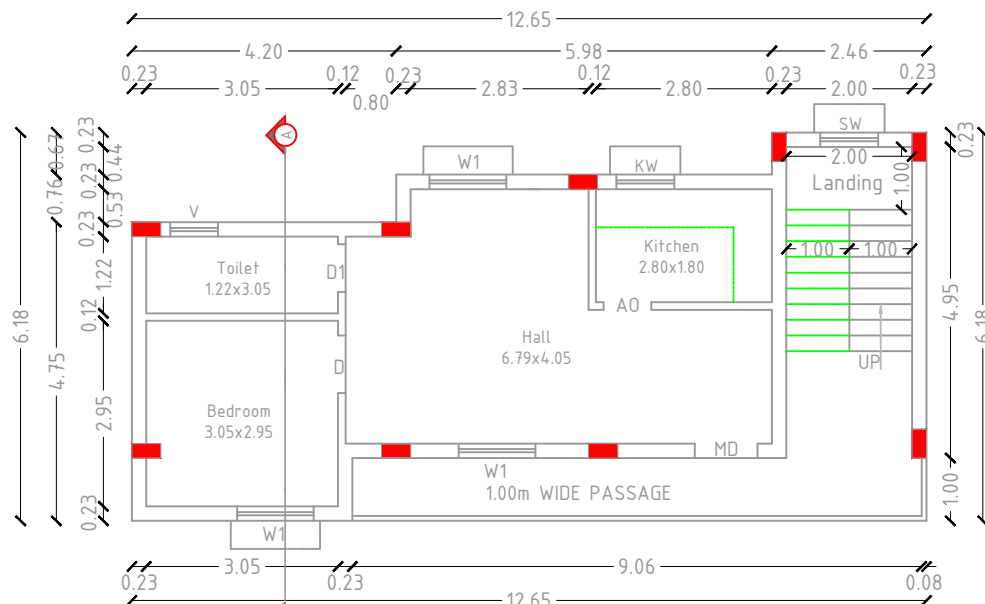
TYPICAL FLOOR PLAN SECOND & THIRD
