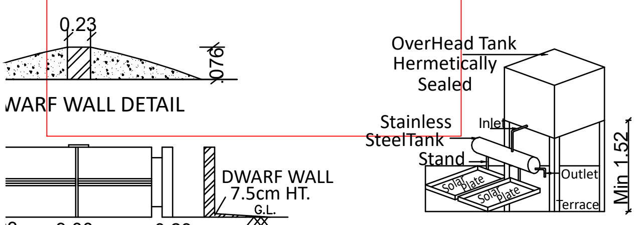
SOLAR WATER HEATING SYSTEM
