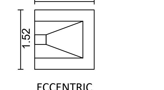
ECCENTRIC FOUNDATION PLAN
