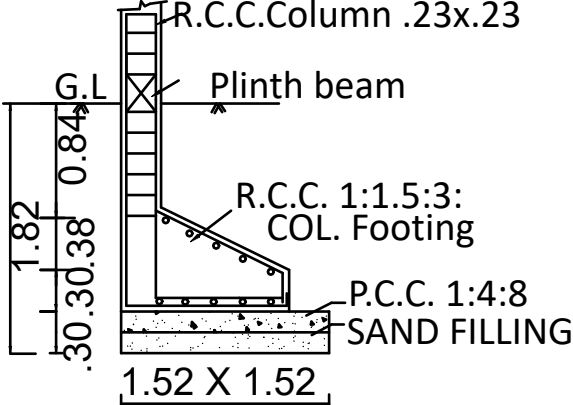
FOUNDATION DETAIL
