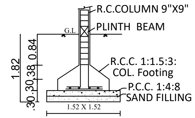
FOUNDATION DETAIL
