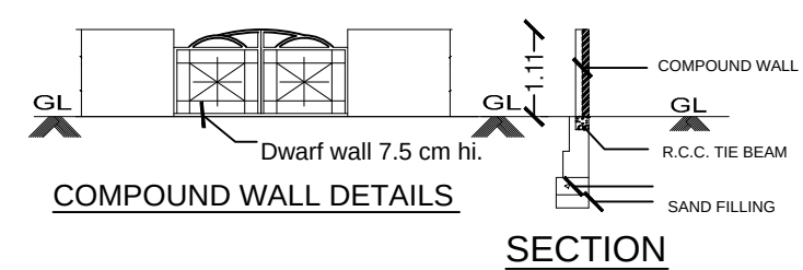
COMPOUND WALL DETAILS
