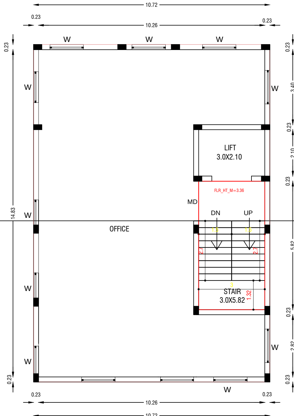
FIRST FLOOR PLAN (PROPOSED)
