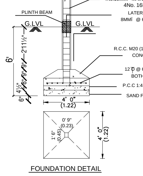
FOUNDATION DETAIL
