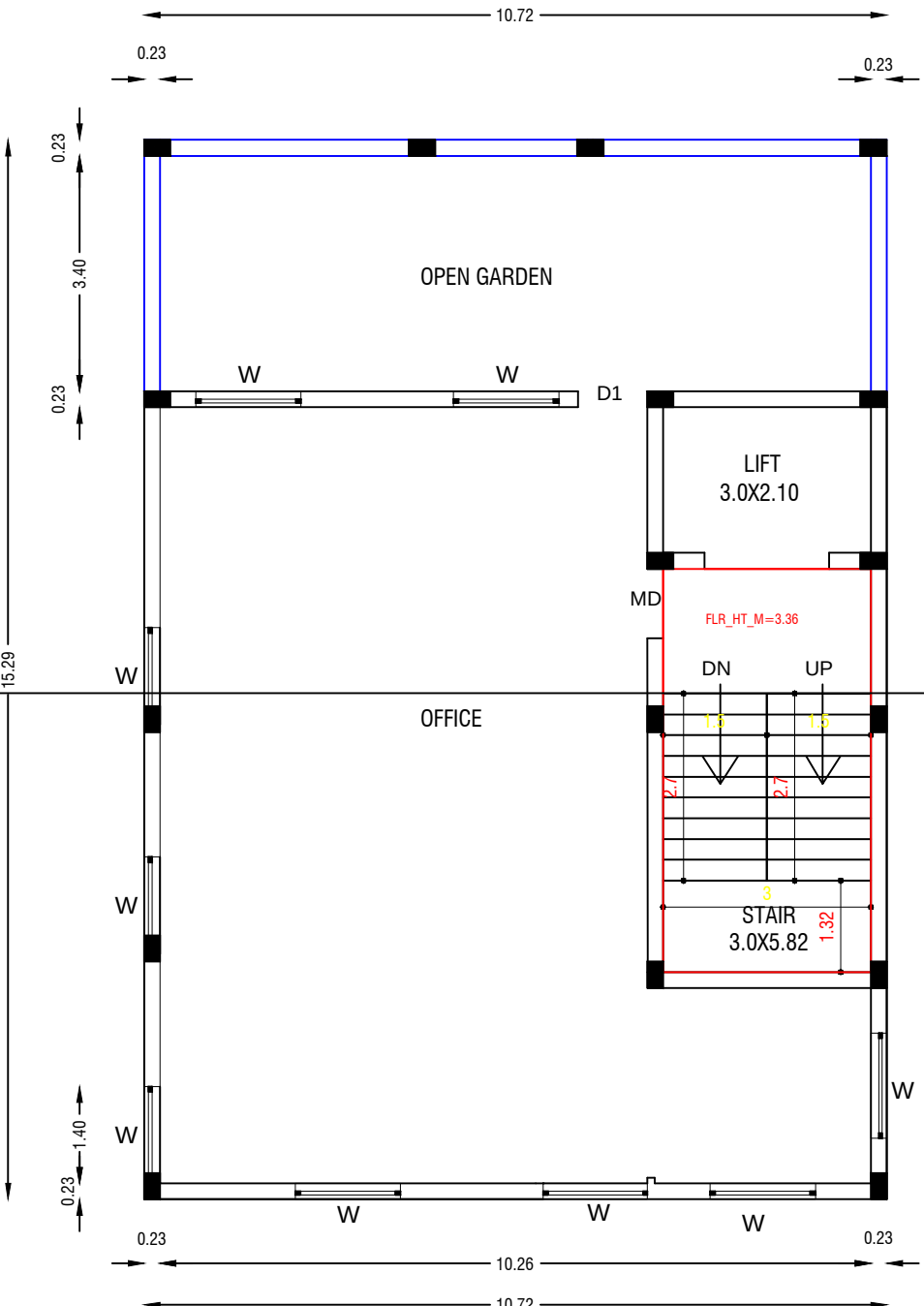
SECOND FLOOR PLAN (PROPOSED)
