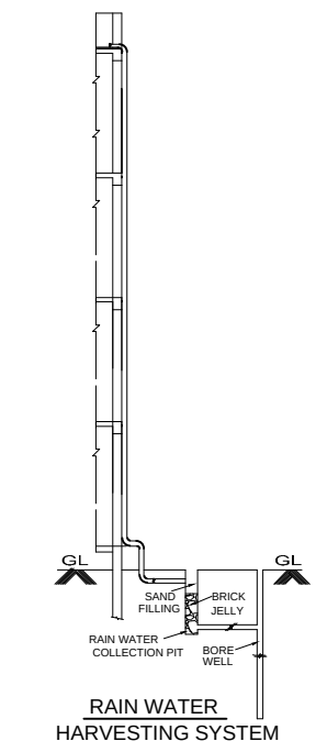
RAIN WATER HARVESTING SYSTEM
