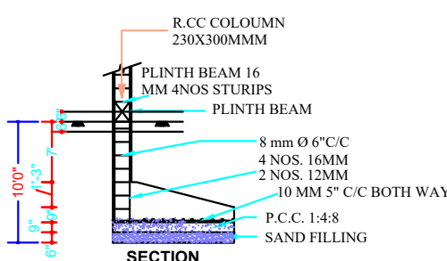
DETAIL OF COLUMN C1,C2
