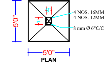
DETAIL OF COLUMN C1,C2
