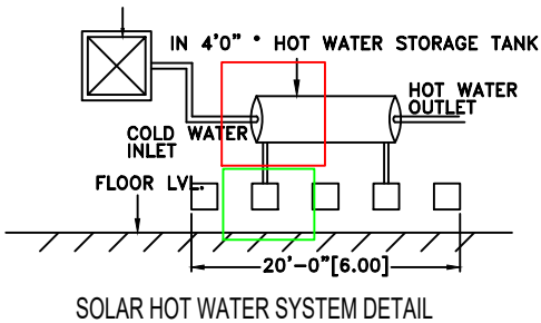
SOLAR HOT WATER SYSTEM DETAIL
