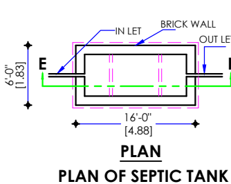
PLAN OF SEPTIC TANK
