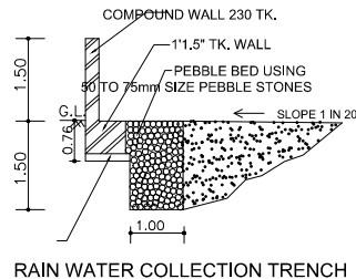
RAIN WATER COLLECTION TRENCH
