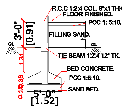
COLUMN FOUNDATION
