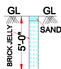
PERCULATION PIT
