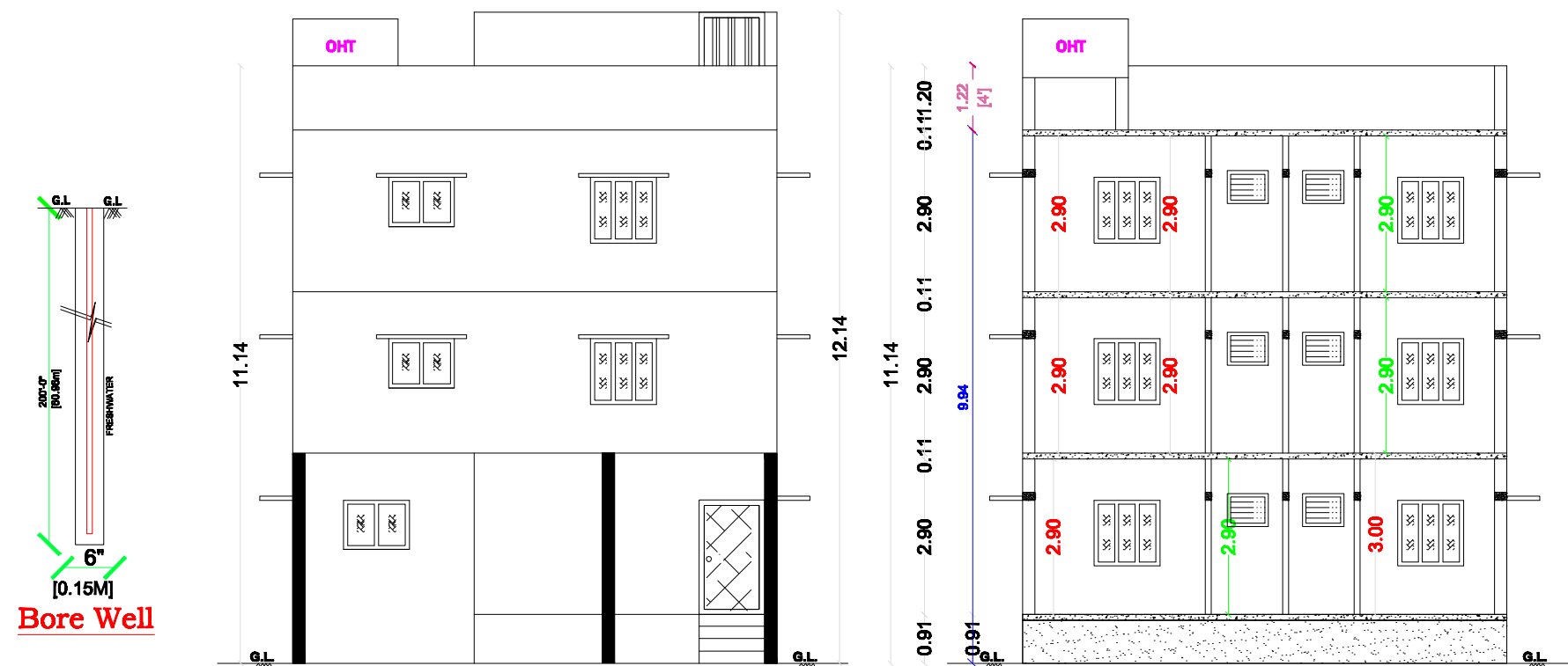
FRONT ELEVATION
